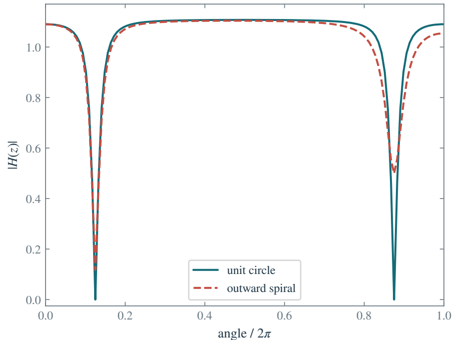
Transfer-function magnitude
