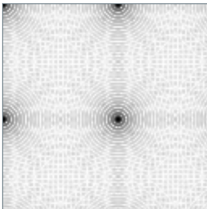
\alpha = 1.8
