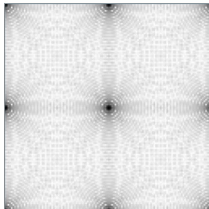
\alpha = 2.0
