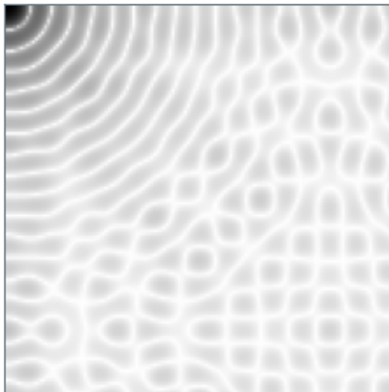
\alpha = 1.2
