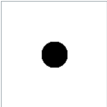
\alpha = 1.0
