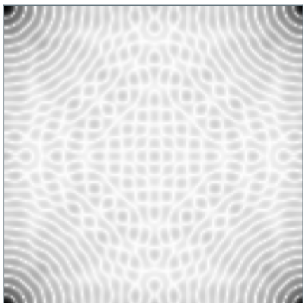
\alpha = 1.6
