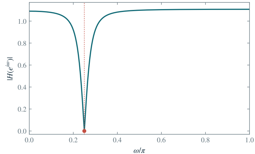
Frequency response
