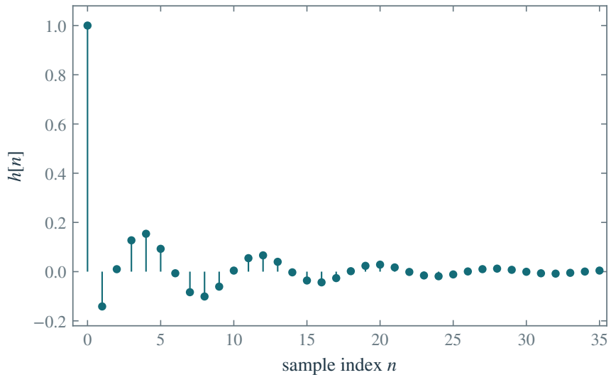
Impulse response
