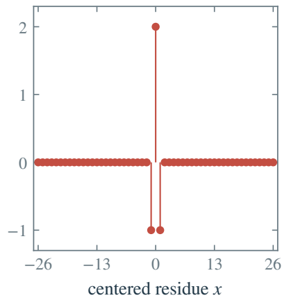
Wavelet \psi
