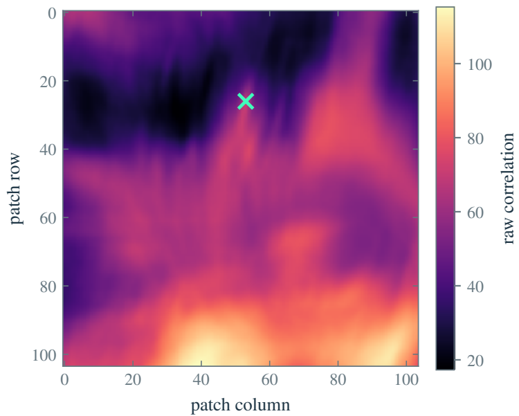
Raw correlation
