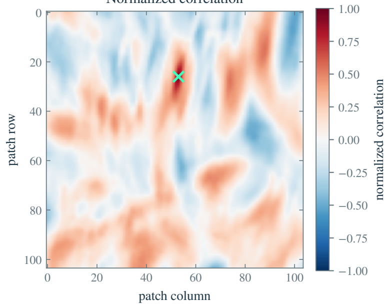
Normalized correlation
