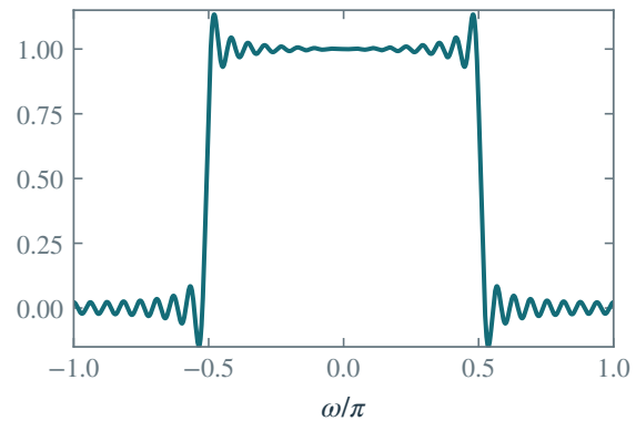
FIR frequency response
