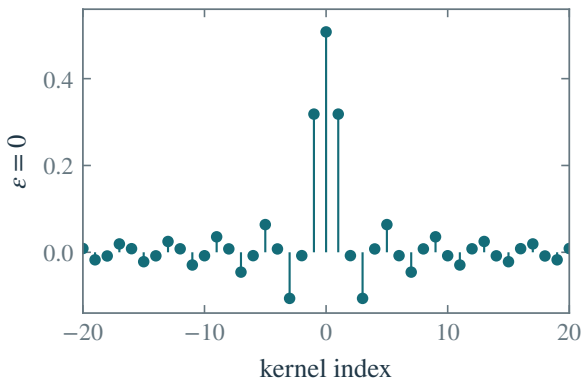
Impulse response
