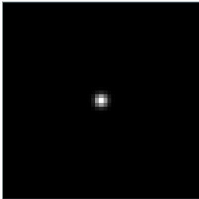
\sigma = 1 pixels
