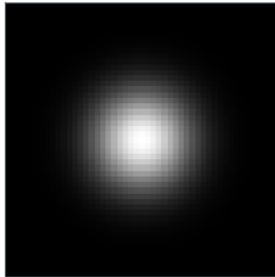
\sigma = 6 pixels
