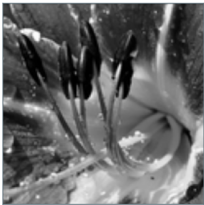
smoothed image
