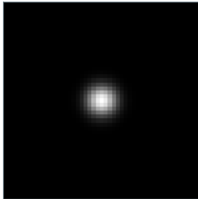
\sigma = 2.5 pixels
