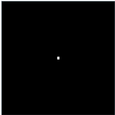
\sigma = 0.3 pixels
