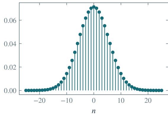
Impulse response
