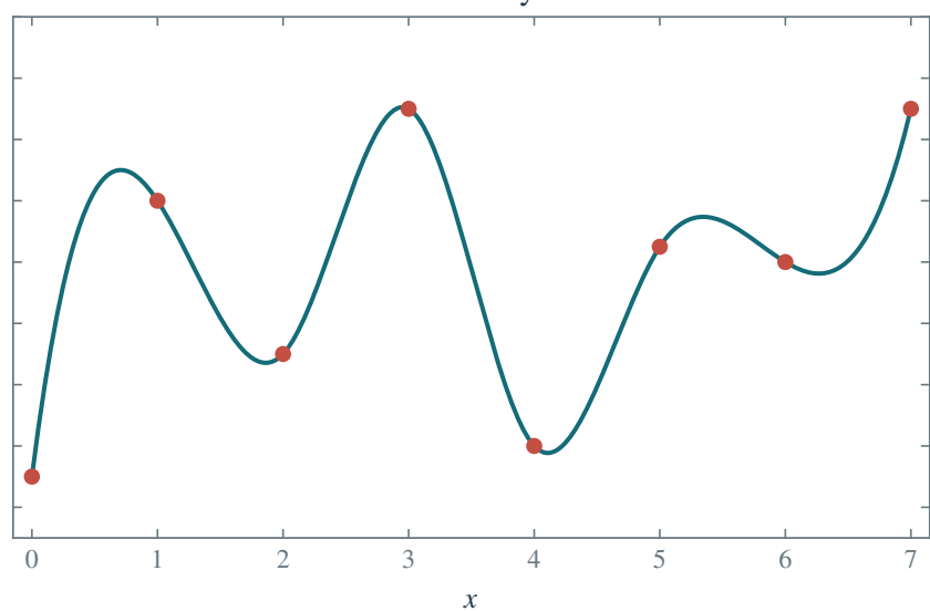
Not-a-knot boundary conditions
