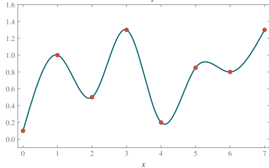
Natural boundary conditions
