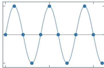
\text{Im } \chi_3
