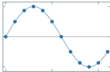
\text{Im } \chi_1
