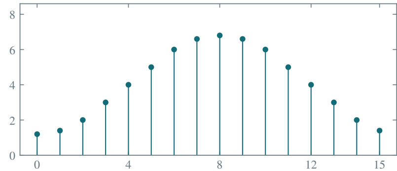
Circular convolution
