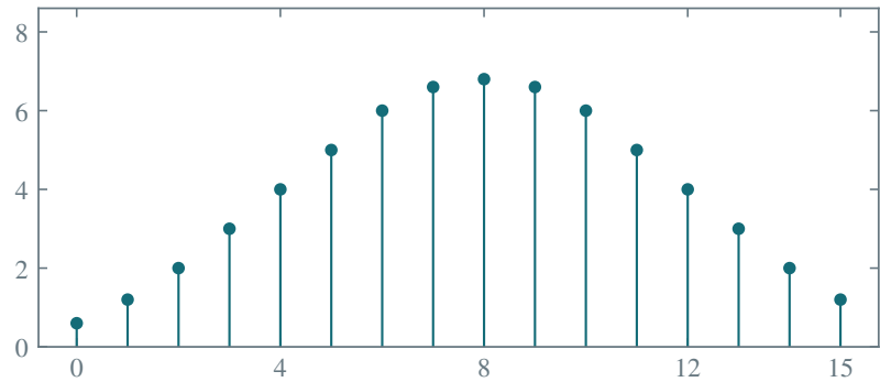
Zero-extended linear convolution
