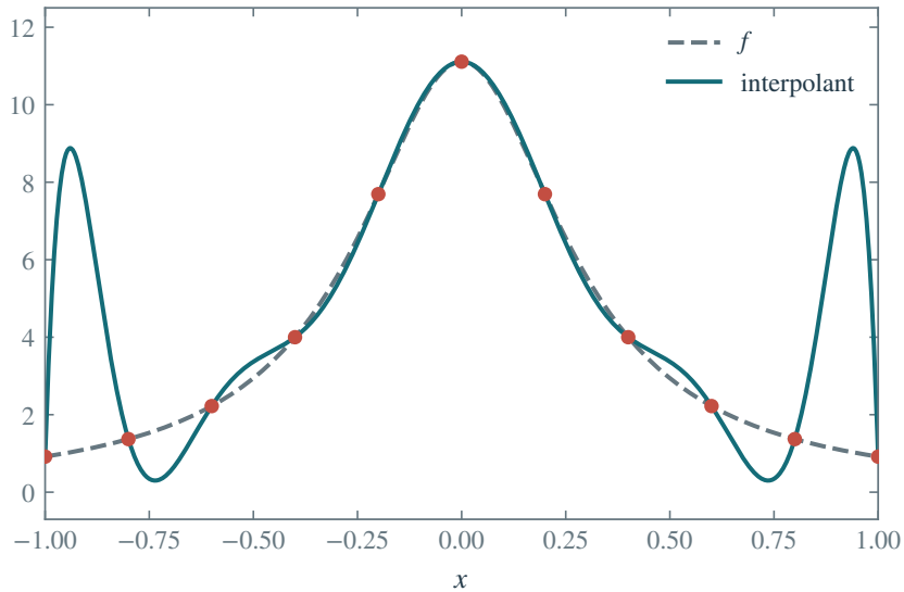
Equally spaced nodes
