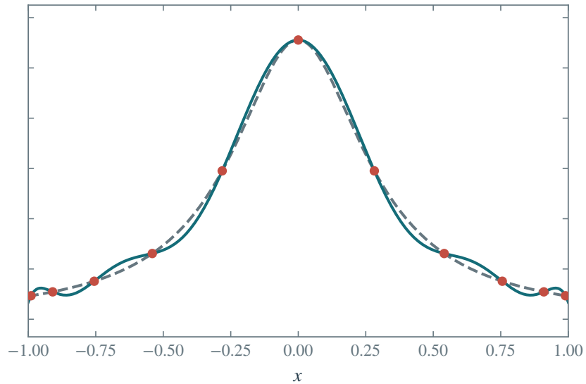
Roots of T_{11}
